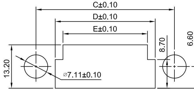
PANEL CUT-OUT PANET THICKNESS 1.27mm
