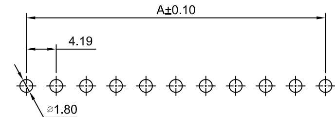
P.C.B LAYOUT TOLERANCE:±0.05
