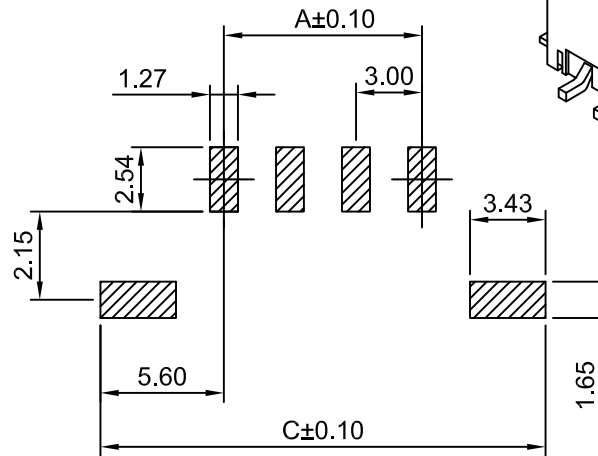
P.C.B LAYOUT TOLERANCE:±0.05
