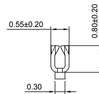
SEC: C-C
