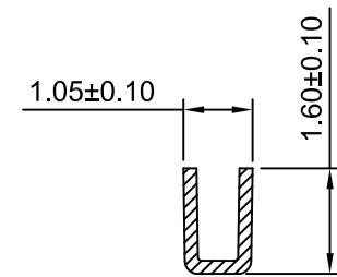
SEC:C-C
