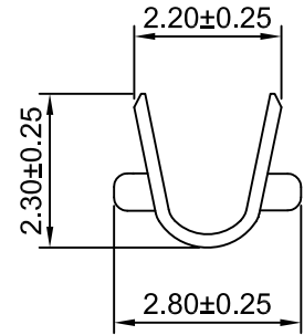
SEC: C-C
