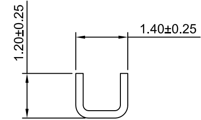
SEC:C-C
