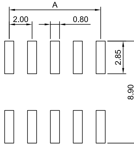
PCB LAYOUT
