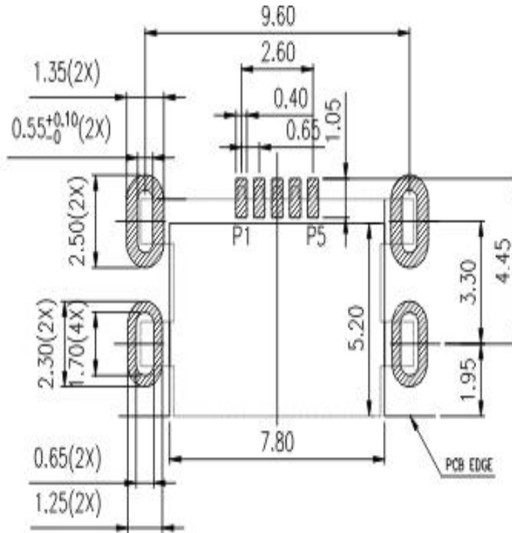
RECOMMENDED PCB LAYOUT(TOP VIEW) GENERAL TOLERANCES:±0.05
