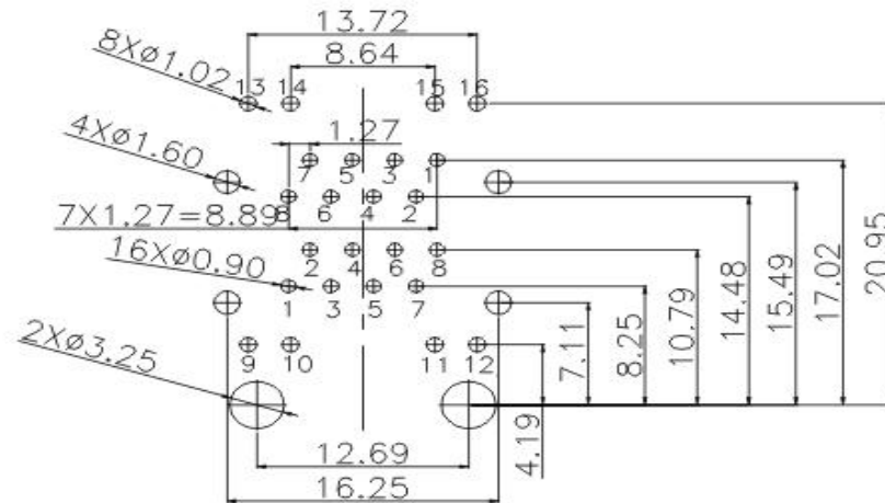
Recommended PCB Layout (PCB TOLERANCE±0.05)
