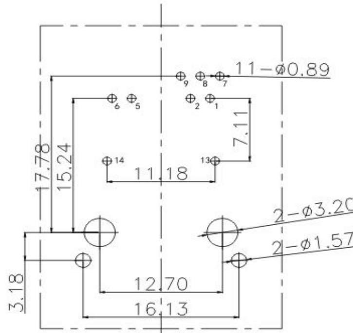
Recommended PCB Layout (PCB TOLERANCE±0.05)
