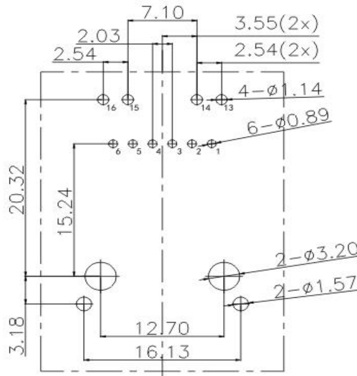
Recommended PCB Layout (PCB TOLERANCE ±0.05)
