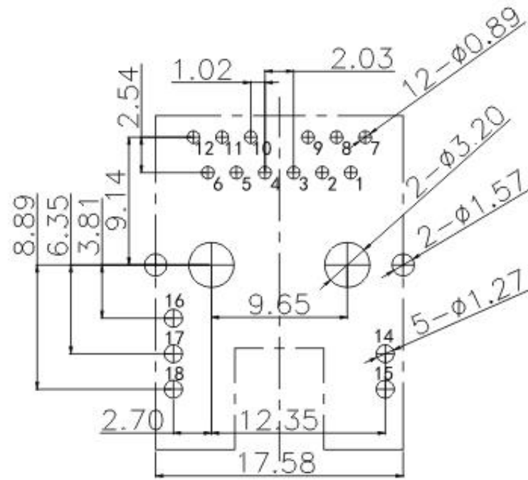
Recommended PCB Layout (PCB TOLERANCE±0.05)
