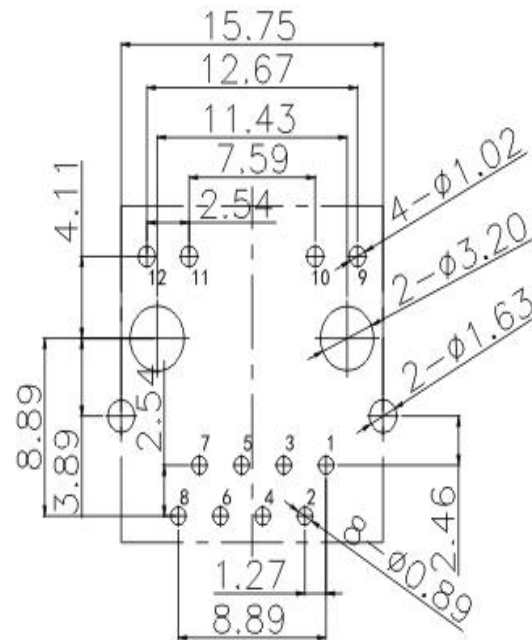
Recommended PCB Layout (PCB TOLERANCE \pm 0.05)
