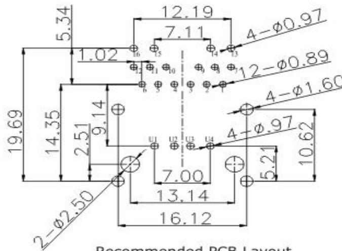
Recommended PCB Layout (PCB TOLERANCE \pm 0.05)
