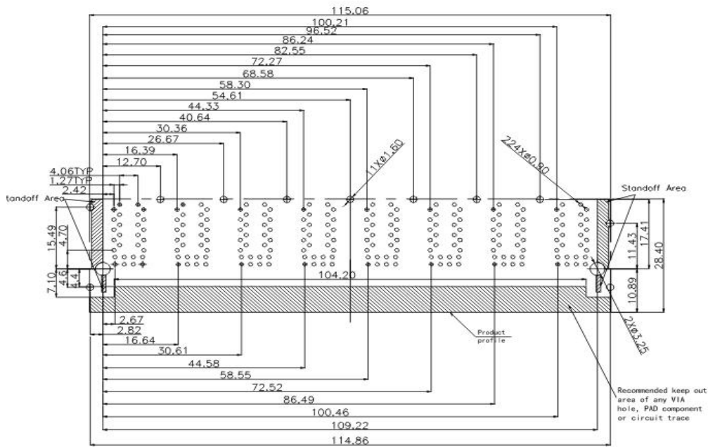
Recommended PCB Layout (PCB TOLERANCE±0.05)
