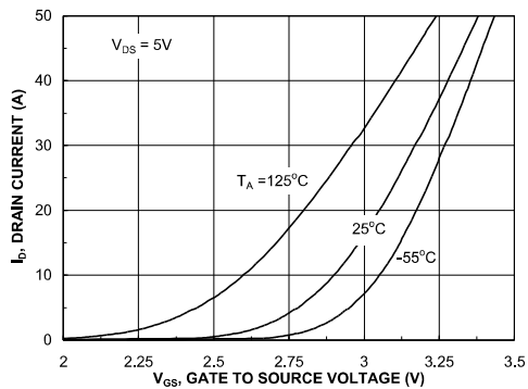
Figure 5. Transfer Characteristics.
