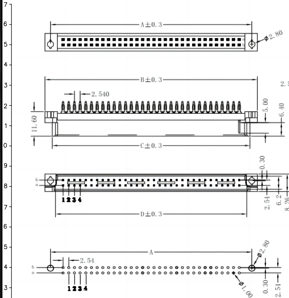
PCB LAYOUT(RECOMMENDED)
