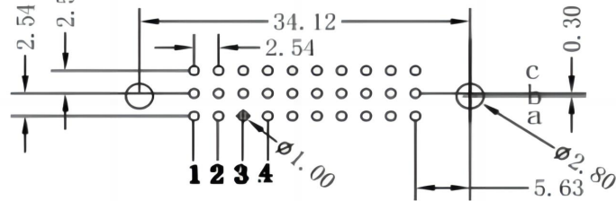
PCB LAYOUT(RECOMMENDED)
