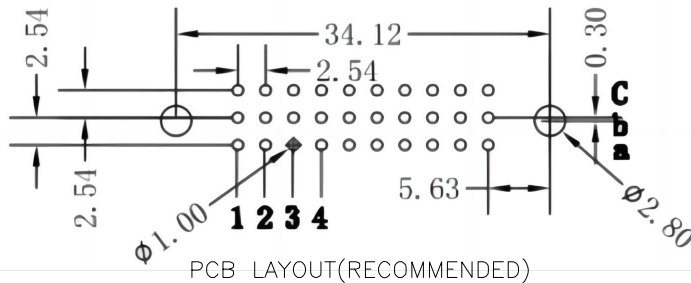
PCB LAYOUT(RECOMMENDED)
