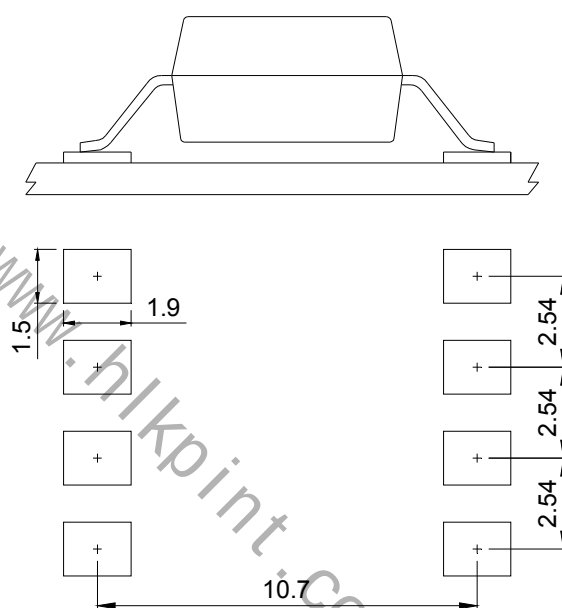
8-pin L
