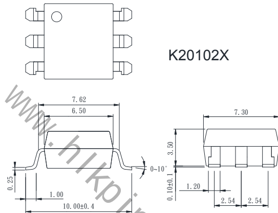
2. Surface mount type.
